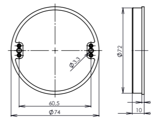
spacer ring VK1
