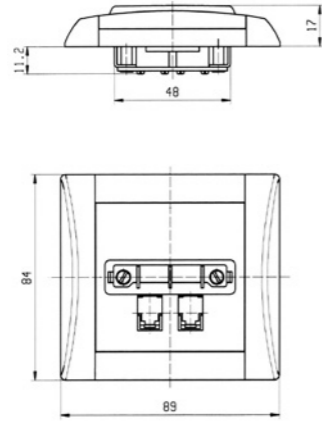
telephone outlet
