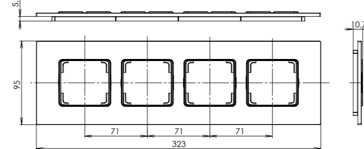
fourfold frame horizontal
