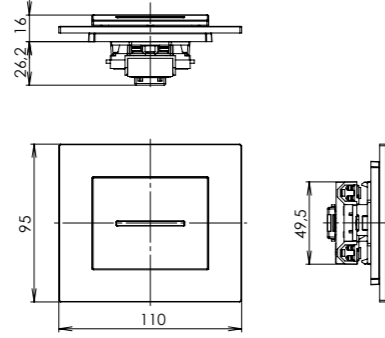
switch with single cover with backlighting
