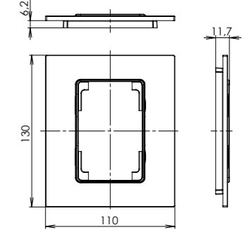
double outlet frame
