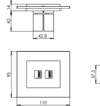
modular outlet USB with charger
