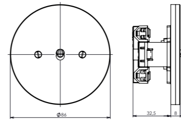
house switch with frame arrangement 1, 2, 6, 7, 1/0
