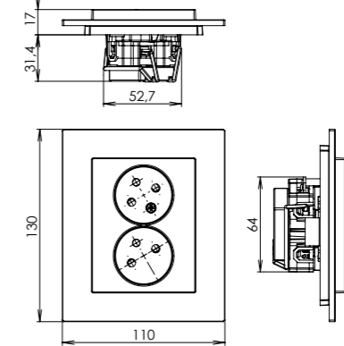
double outlet with safety shutters and overvoltage protection (audible alarm or light indication)
