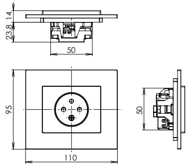
single outlet with safety shutters
