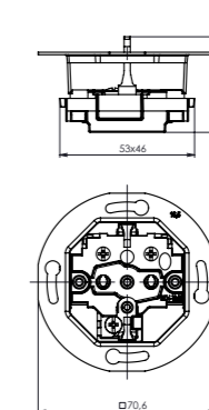
schuko single outlet
