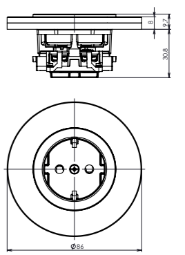
schuko single outlet with frame
