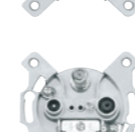
TV+R+SAT outlet through, attenuation 10 dB, 300 mA, 24 V DC for coaxial cables of diameter 4.5–8.3 mm designation on the product: ZAR-SAT 10/P3
