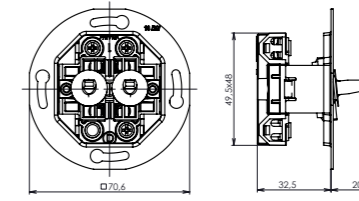
house switch arrangement 5, 6+6, 6/0+6/0
