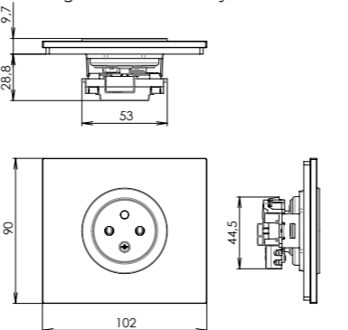
single outlet with safety shutters
