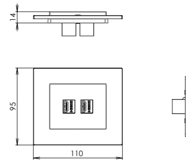
modular data outlet HDMI, USB, RJ45
