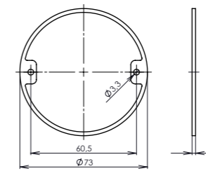
spacer ring VK2
