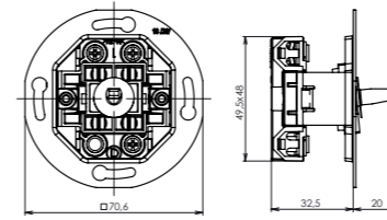
house switch arrangement 1, 2, 5, 6
