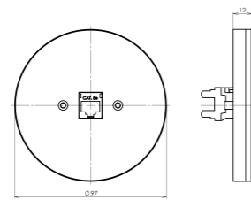
PC, RJ 45 outlet glass
