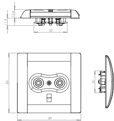
protective bonding outlet
