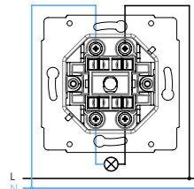
switch arrangement 2 (twopole switch)
