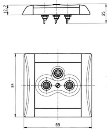
AUDIO-VIDEO outlet
