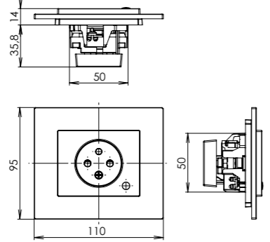
single outlet with safety shutters and overvoltage protection (light indication)
