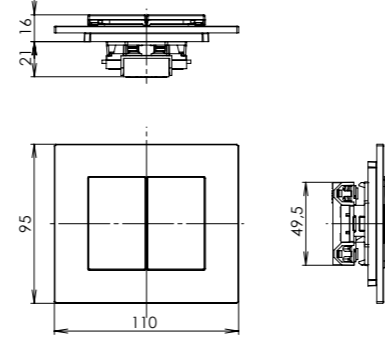
switch with double cover
