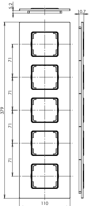
fivefold frame vertical
