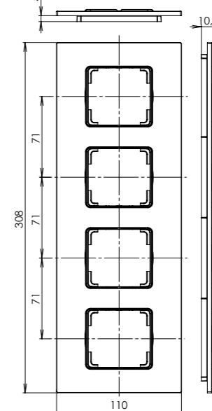
fourfold frame vertical
