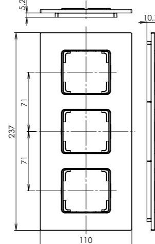
triple frame vertical
