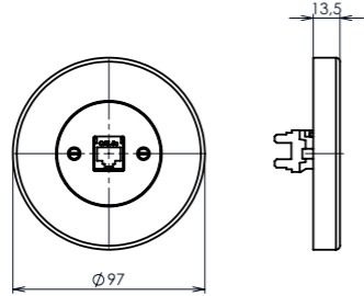
PC, RJ 45 outlet
