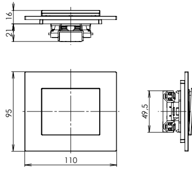
switch with single cover
