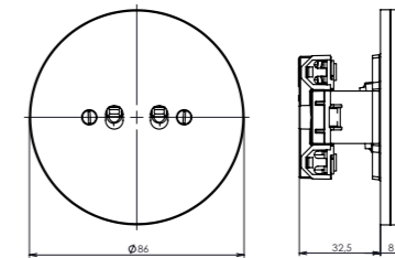
house switch with frame arrangement 5, 6+6, 6/0+6/0
