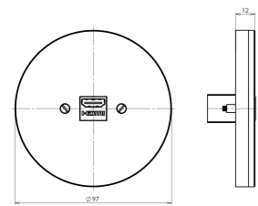
HDMI, USB,TV,SAT outlet glass
