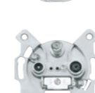
TV+R+SAT outlet terminal, attenuation 1 dB, 300 mA, 24 V DC for coaxial cables of diameter 4.5–8.3 mm designation on the product: ZAR-SAT 1.4/K
