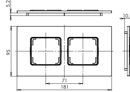
double frame horizontal
