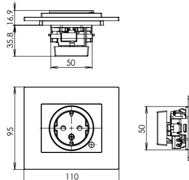
single outlet with safety shutters and overvoltage protection (light indication and audible alarm)
