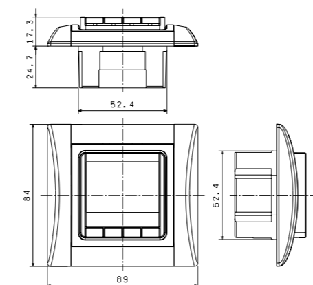
digital thermostat DSE 4T
