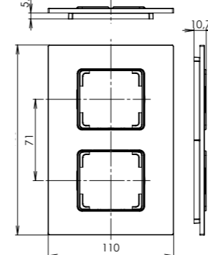
double frame vertical
