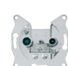
TV+R outlet through branching attenuation 14 dB for coaxial cables of diameter 4.5–8.3 mm designation on the product: ZAP 14
