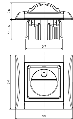
motion sensor STEINEL
