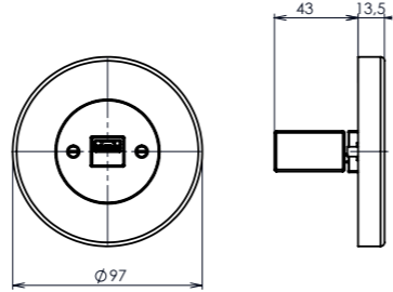
outlet with USB-A charging
