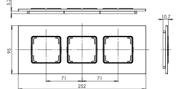
triple frame horizontal
