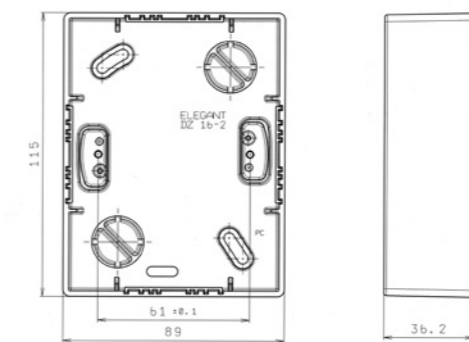
double outlet installation box, on-plaster
